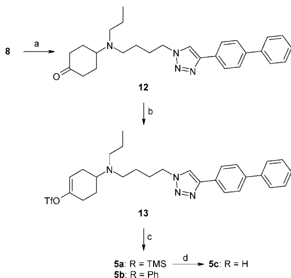
Scheme 2 a
